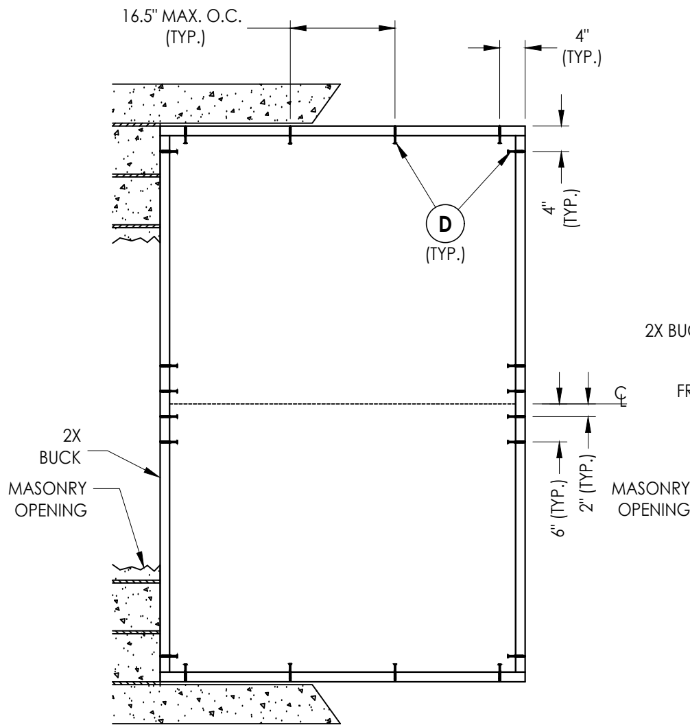
BUCK ANCHORING
