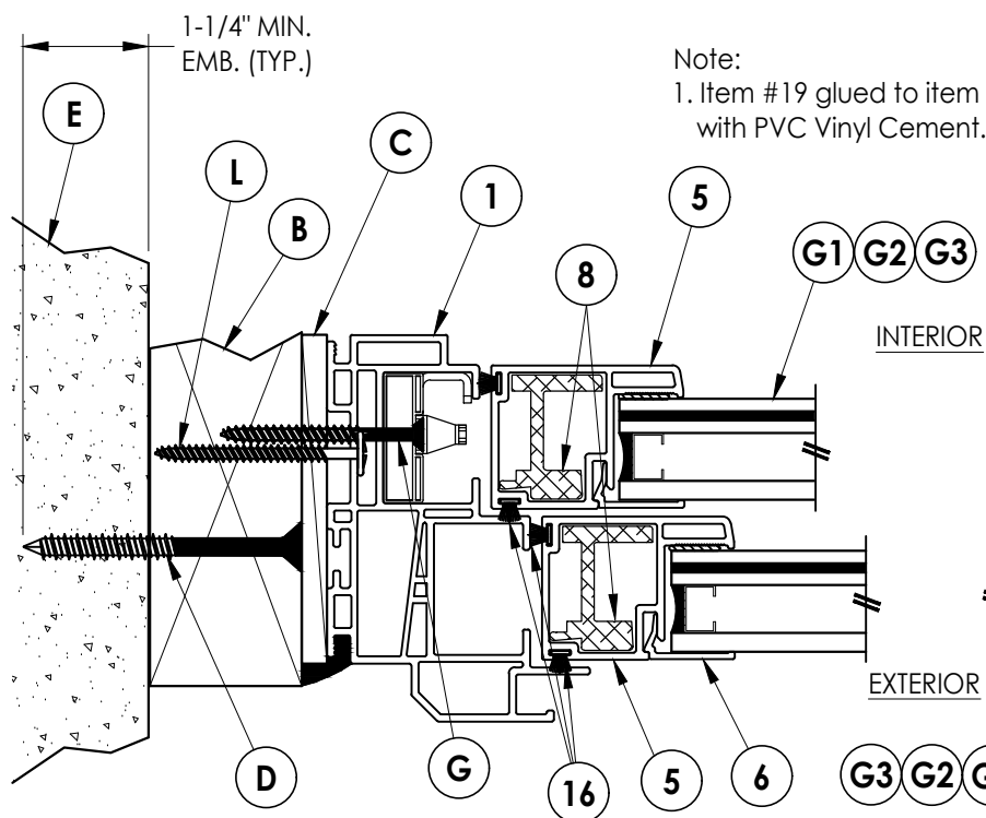
4 4 HORIZONTAL CROSS SECTION Shown w/ 2X buck
