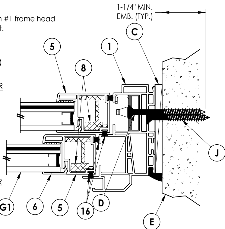
5 4 HORIZONTAL CROSS SECTION Shown direct to masonry
