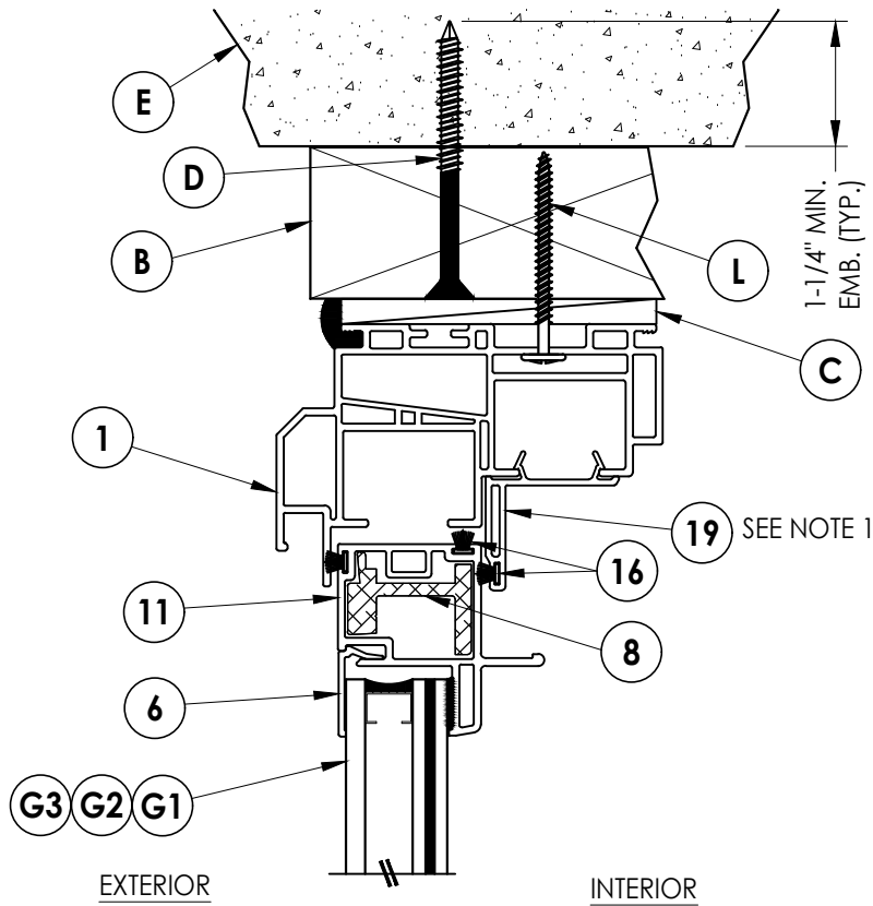
1 4 VERTICAL CROSS SECTION Shown w/ 2X buck
