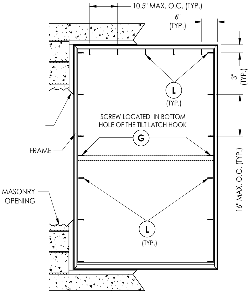
FRAME ANCHORING 2X Buck
