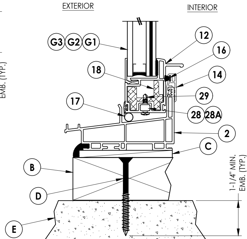
3 4 VERTICAL CROSS SECTION Shown w/ 2X buck
